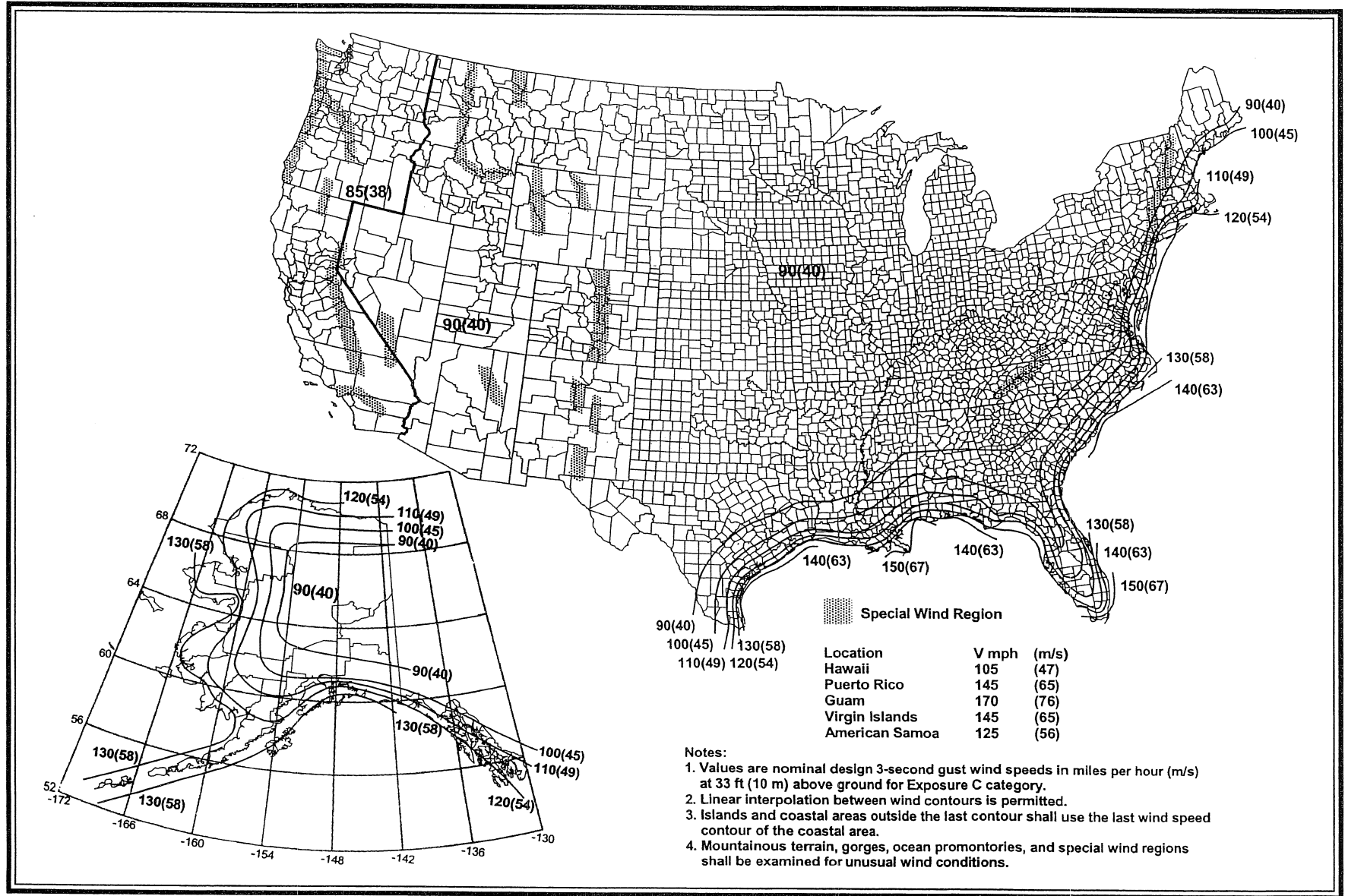
Figure 3.2.2 Basic Wind Speed
